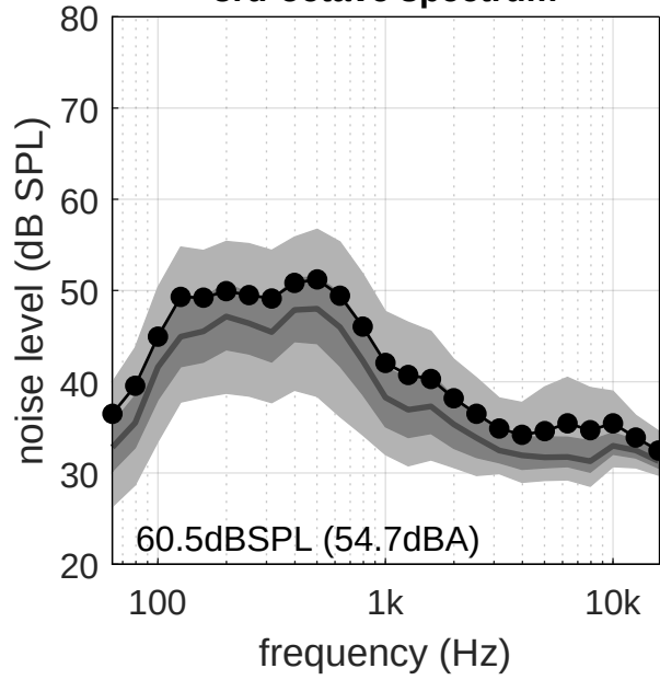
3rd-octave spectrum
