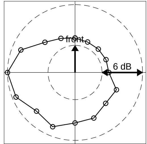
Directional behaviour
